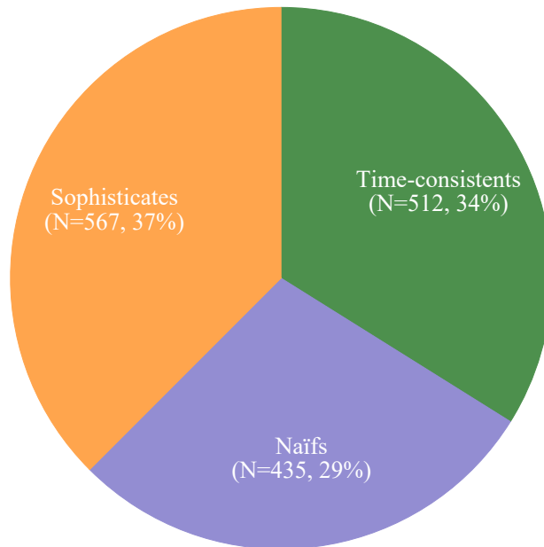
Figure 3: Type distribution
